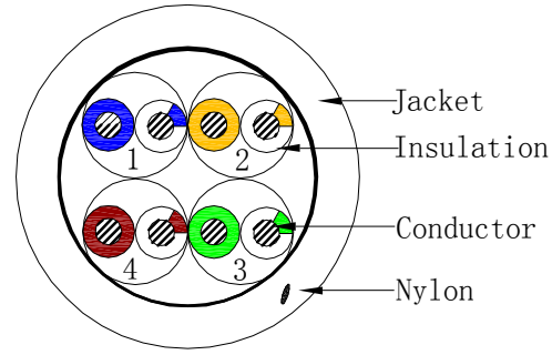
CROSS-SECTION/截面图
