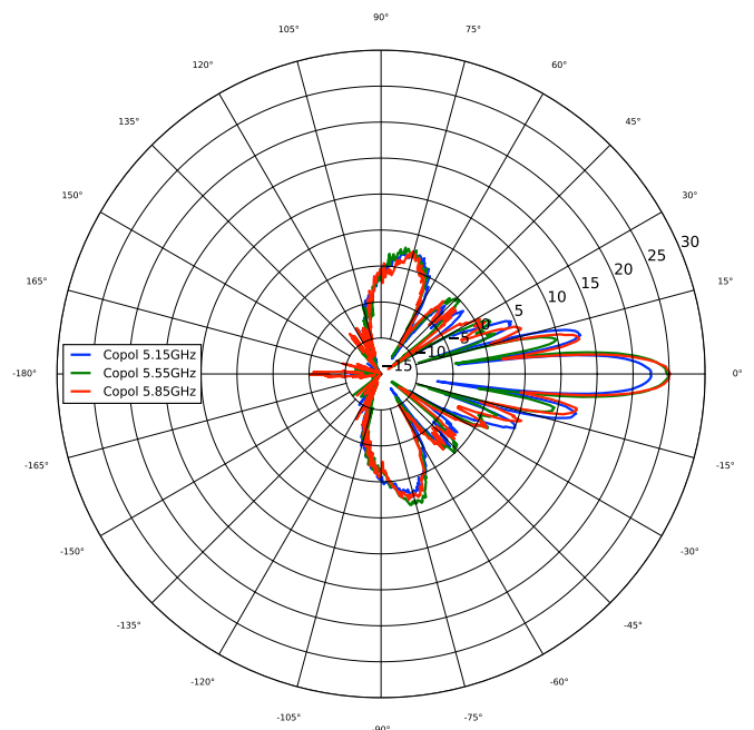
Azimuth, Vertical
