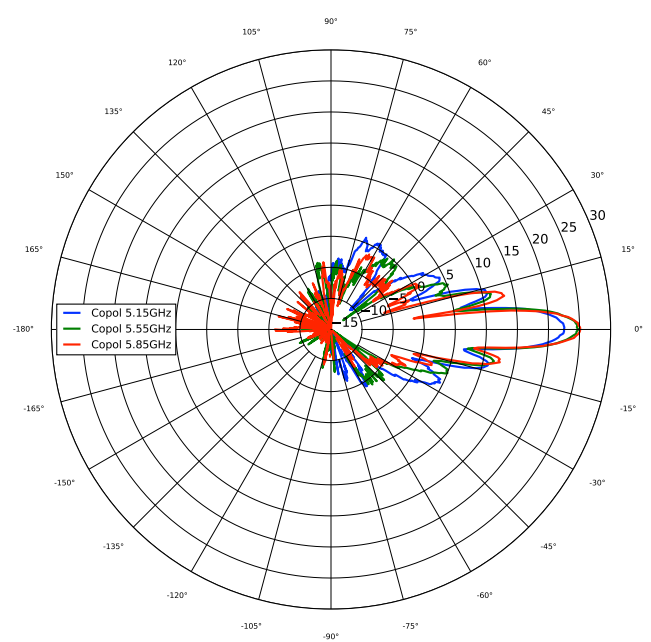
Elevation, Vertical
